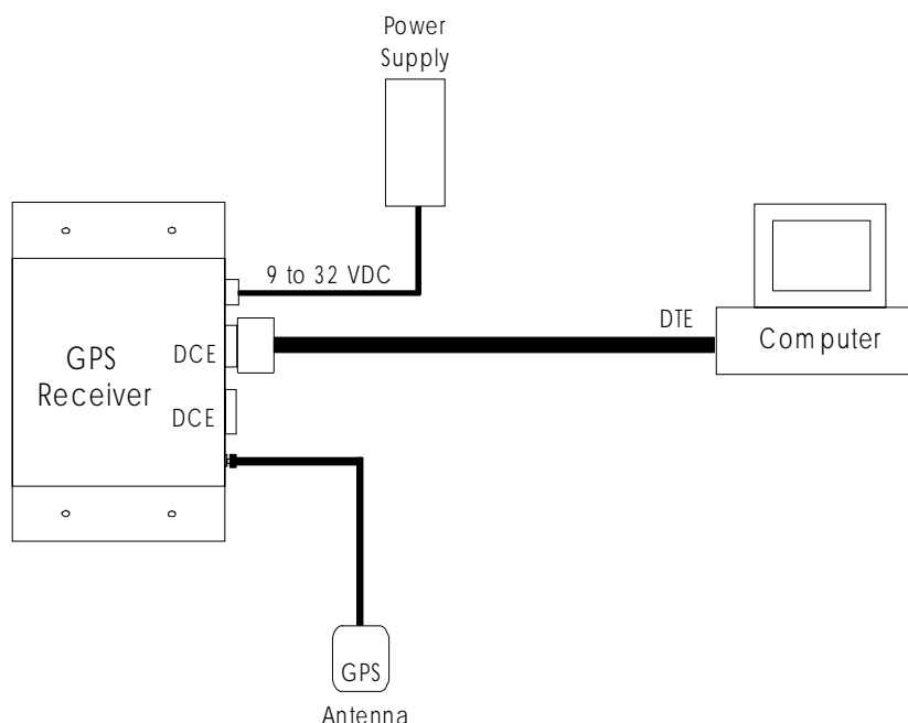
Figure 1-10. Interconnect Diagram
